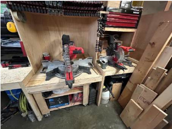
P686 – Mitre Saw Tables (71"W" x 34 "D x 33" H)
