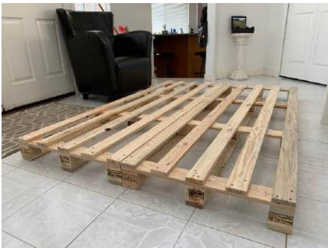
P398 – Bed Frame- (53" W x 74"D x 5"H)
